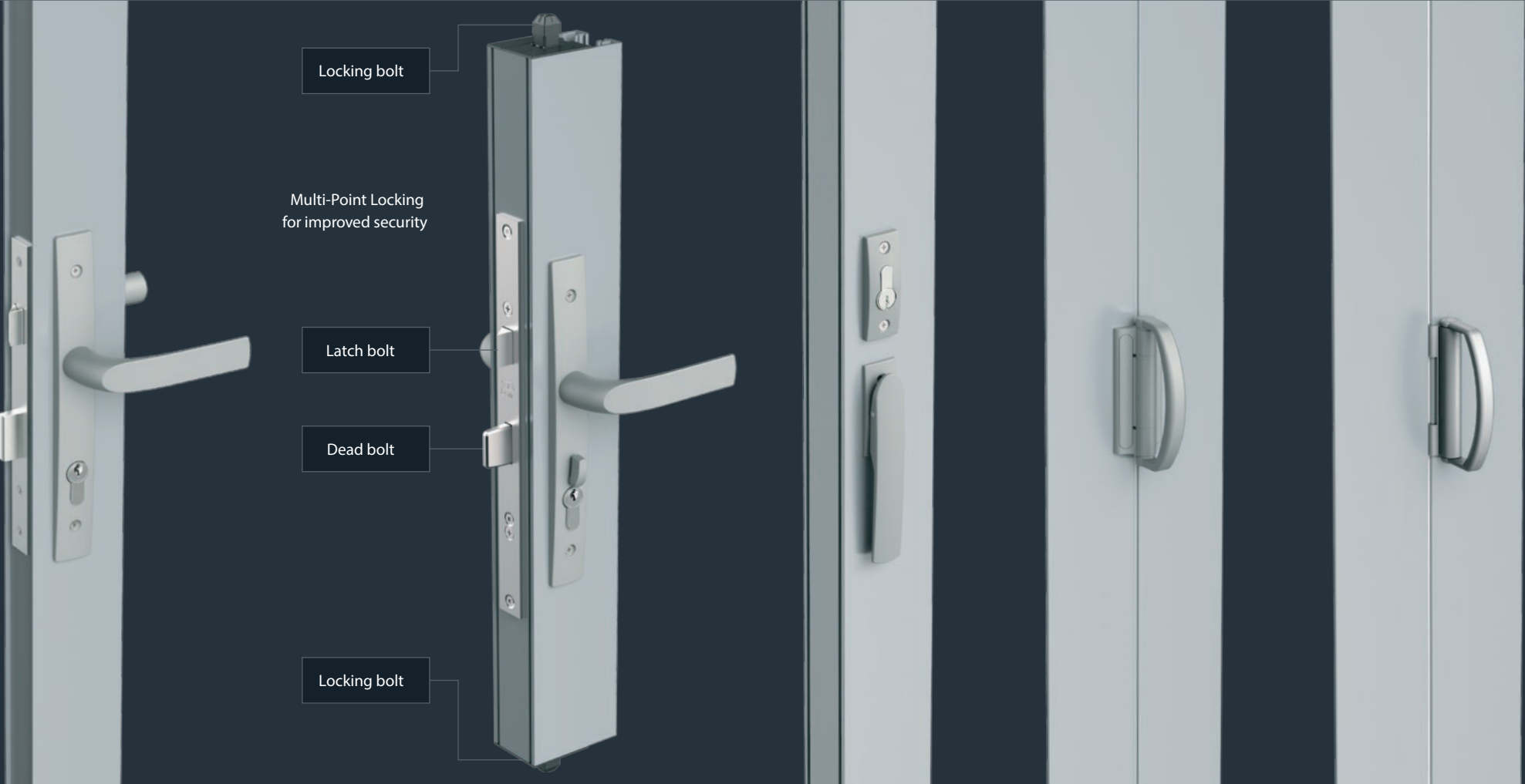
Locking lever
